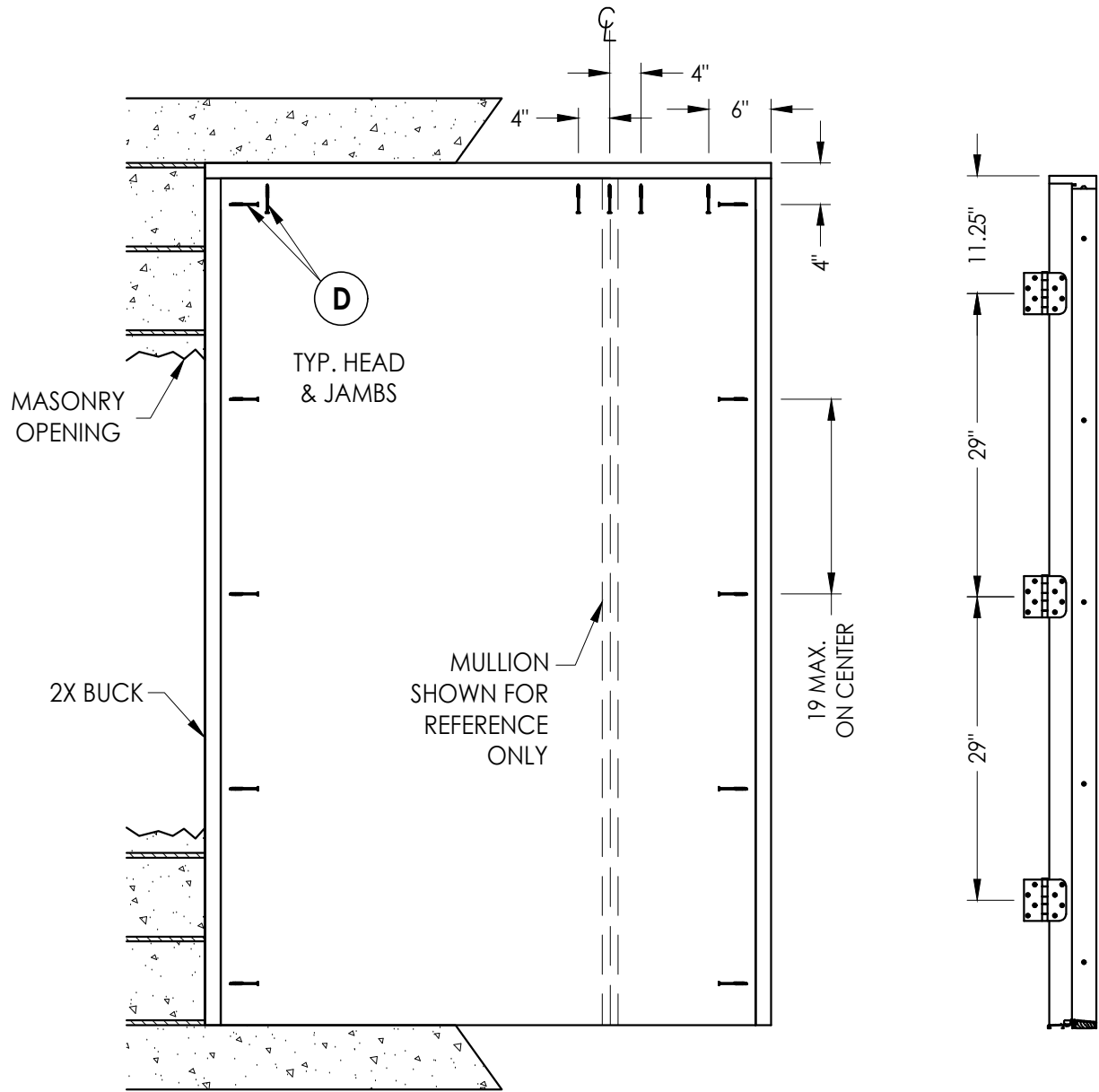
BUCK ANCHORING
