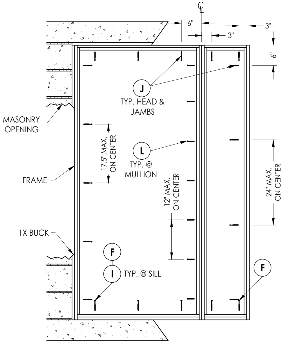
FRAME ANCHORING
