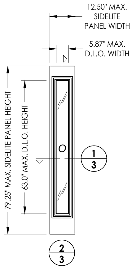
50 SIDELITE PANEL
